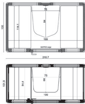
BUSYPOD Large plan section
