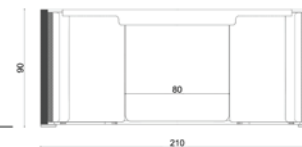
BUSYLOUNGE 2 person plan section
