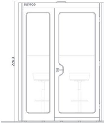
BUSYPOD Medium Meet front view
