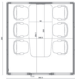
BUSYPOD XLarge Plan section
