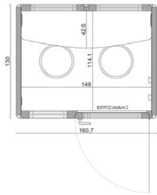
BUSYPOD Medium Meet plan section
