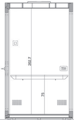
BUSYPOD Medium Work section
