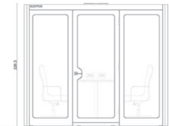
BUSYPOD XLarge Front view
