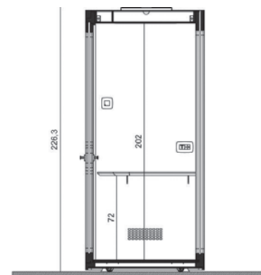
BUSYPOD Plus side view
