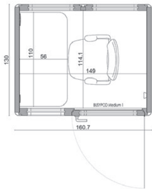
BUSYPOD Medium Work plan section
